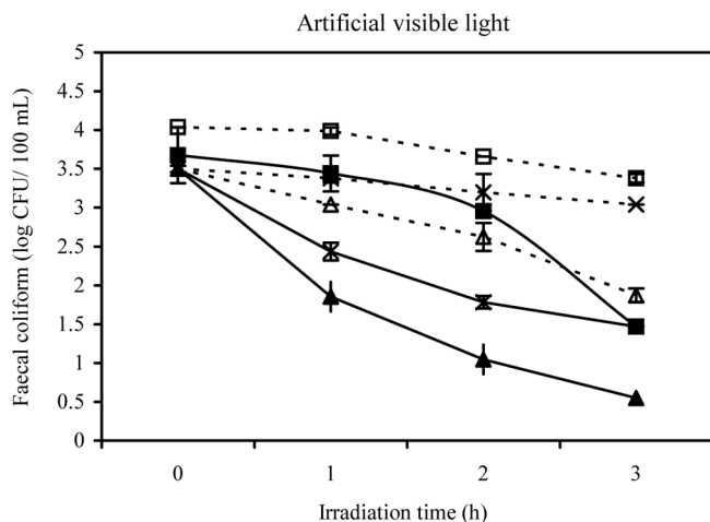
Fig. 3. Faecal coliforms photoinactivation in secondary wastewater effluent by artificial visible light with methylene blue (10 \mu M) at pH values: (---x---) pH 5; (■) pH 7; (▲) pH 9 vs. artificial visible light without methylene blue at pH values: (- -x- -) pH 5; (- -□- -) pH 7; (- -Δ- -) pH 9. Values are means of three replicates.
