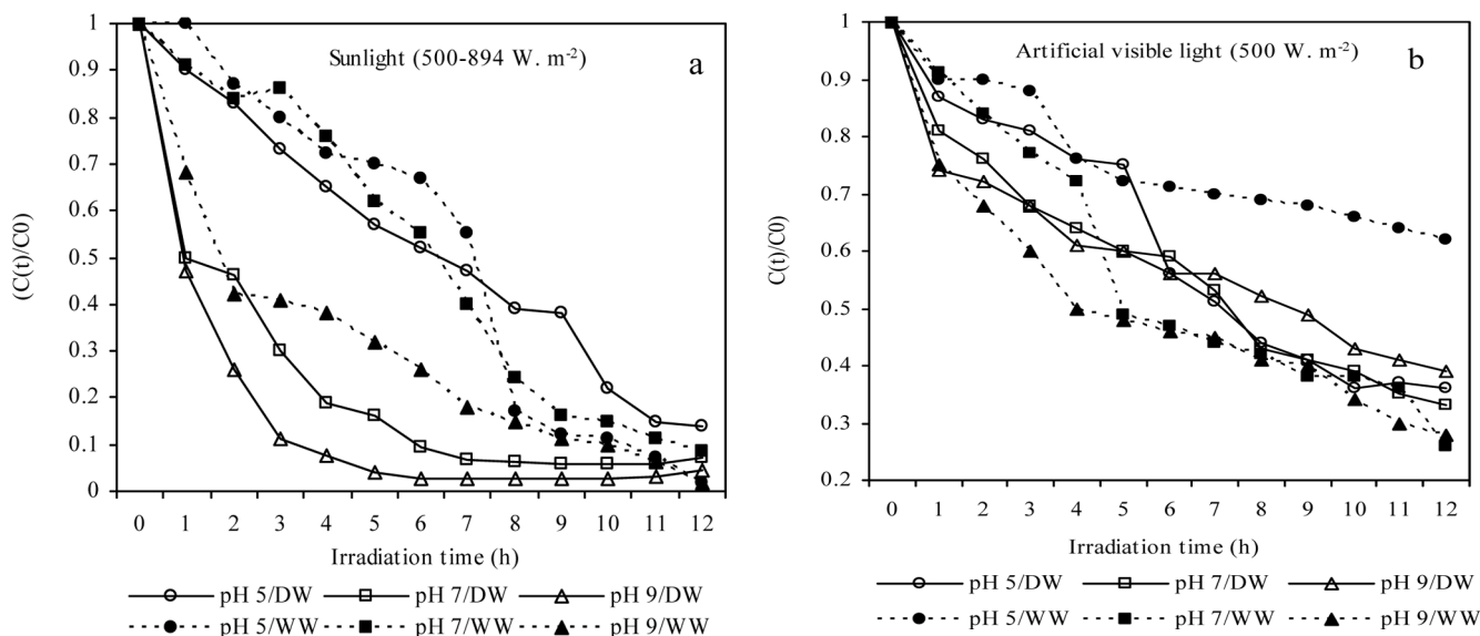
Fig. 5. Methylene blue photobleaching efficiencies at a concentration of 10 \mu\text{M} in distilled water (DW) and secondary wastewater (WW) effluent at different pH values under (a) sunlight and (b) artificial visible light.
