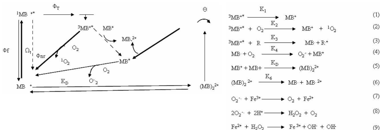
Fig. 4. Methylene blue photochemical reaction routes where \text{MB}^+ , {}^1\text{MB}^{*+} , {}^3\text{MB}^{*+} are methylene blue ground state, singlet and triplet excited states, respectively, \text{MB} . And \text{MB}^{2+} are methylene blue semi-oxidized radicals, respectively, \Omega_1 is light absorption, \Phi_f , \Phi_{nr} , \Phi_T are fluorescence, nonradiative and triplet quantum yield. Reactions (1)–(4) represent the deactivation routes of \text{MB}^{*+} excited state and radical species where (1) is the {}^3\text{MB}^{*+} spontaneous decay, (2) is the reaction of {}^3\text{MB}^{*+} with molecular oxygen, (3) is the redox suppression of {}^3\text{MB}^{*+} by reducing agents, (4) is the oxidation of \text{MB} by molecular oxygen returning the ground state dye and forming superoxide, (5) is the ground state dimerization constant, (6) is the redox suppression of ( {}^3\text{MB}^{*+} ----- \text{MB} ). after exciting ground state dimers, (7)–(9) are Fenton reactions. The relative position of the species presented in this scheme does not represent their actual energy level. Modified from [38] reported by Tardivo et al. [49].
