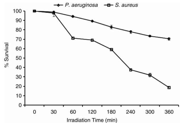
Figure 2 | Effect of continuous irradiation on (◇) P. aeruginosa and (□) S. aureus cell survival in the absence of PSs (light control).
